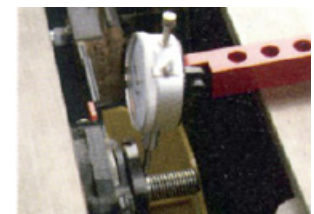
Saw Arbor Shaft Run-out
