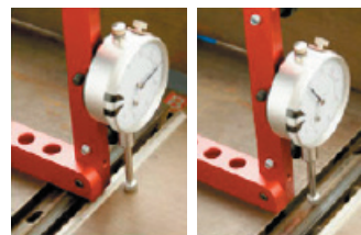
Jointer Depth of Cut & Joiner Knife Position
